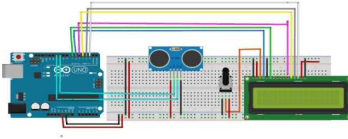
Fig.2 Schematic diagram
