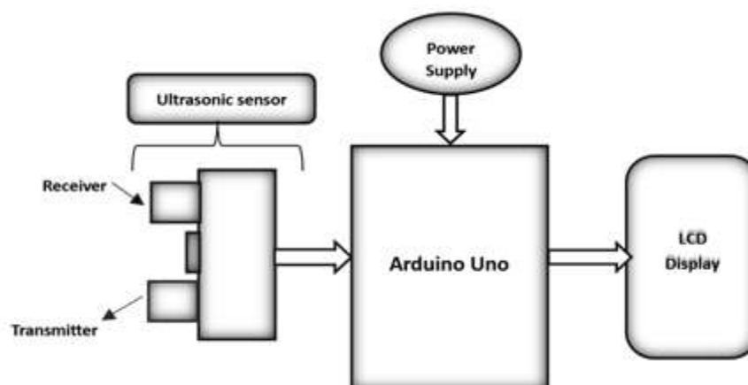
Fig.1 Block diagram
